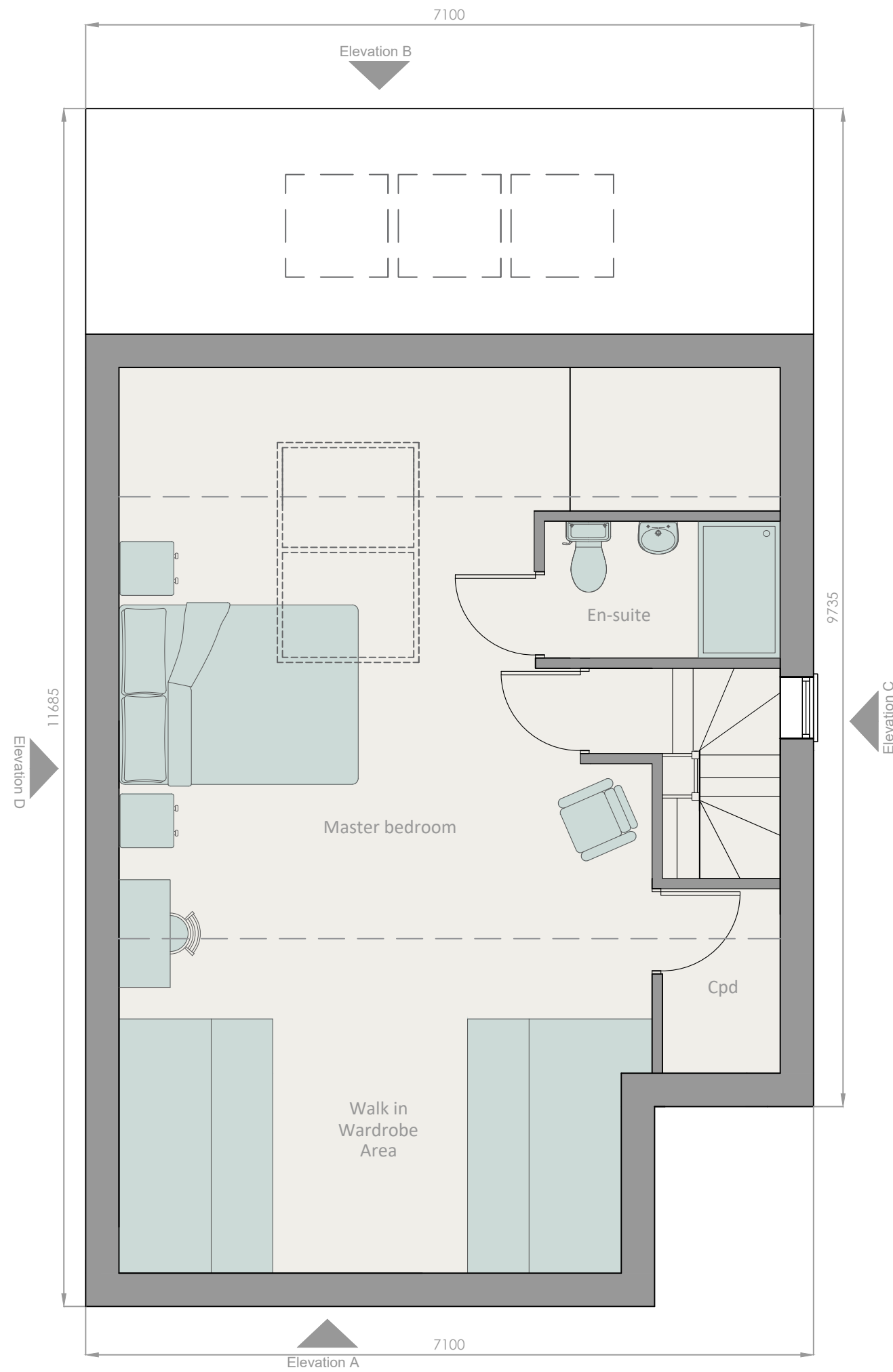
1 The Oakwood Attic Floor Plan 1:50
