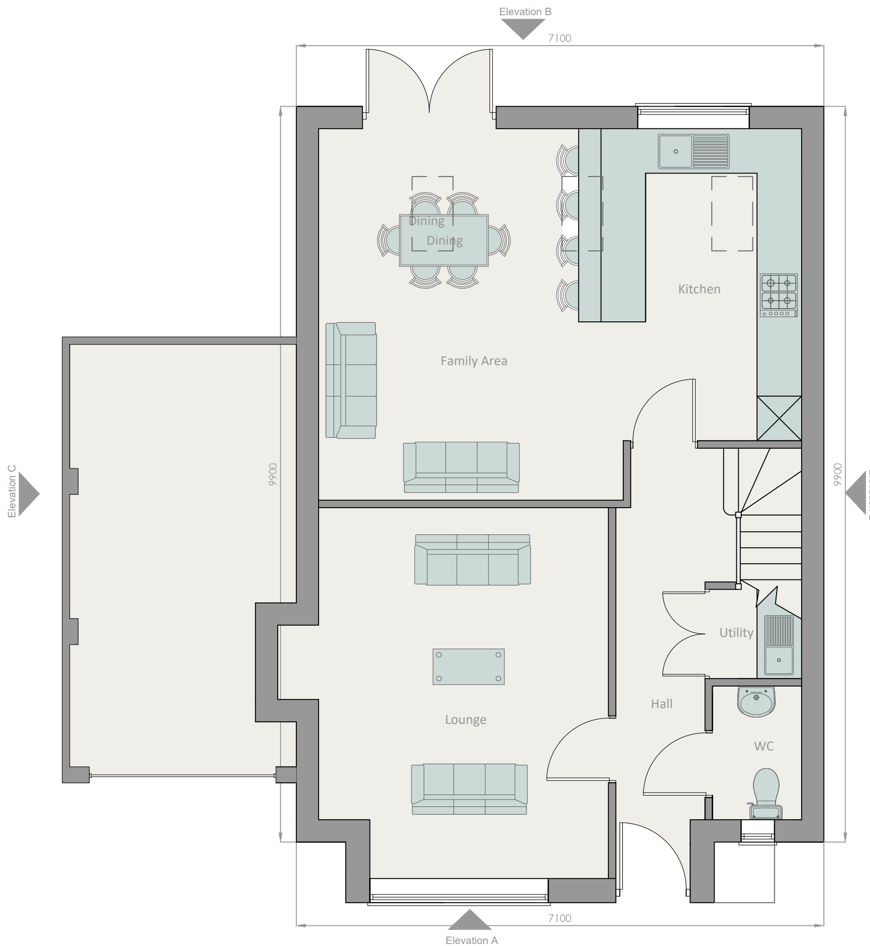
1 The Hathaway Ground Floor Plan 1:50
