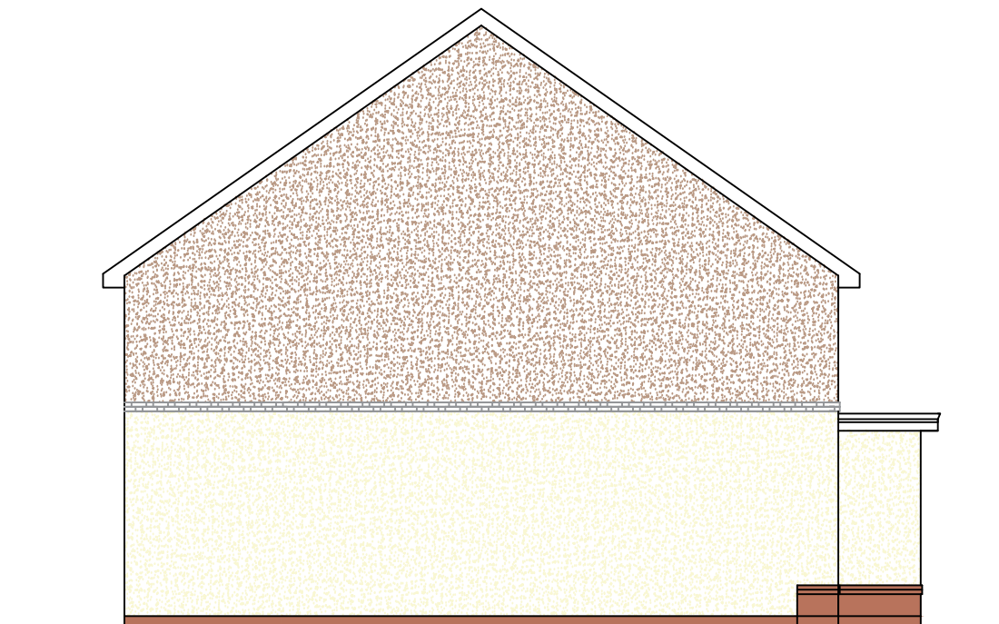
4 The AF1 & AF2 Side Elevation D 1:100
