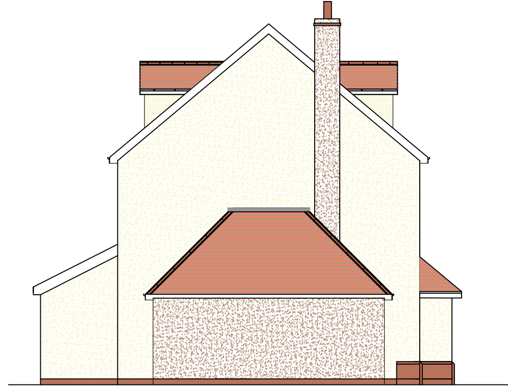
4 The Hathaway Side Elevation D 1:100
