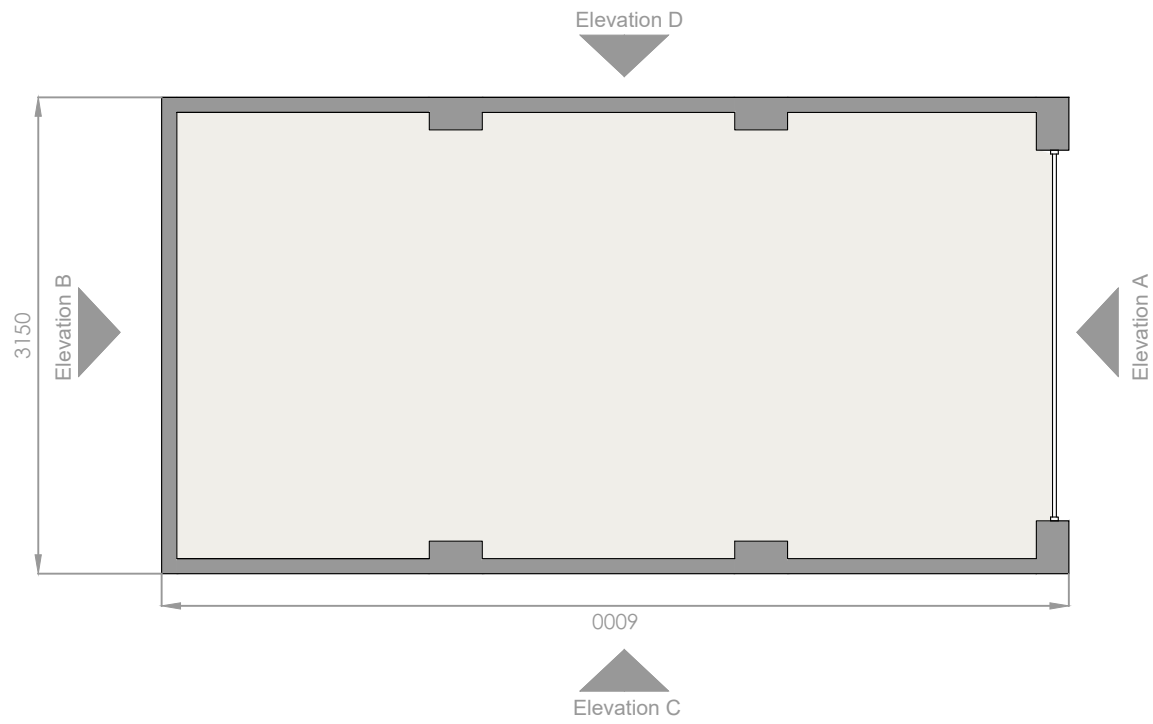
1 Garage Floor Plan 1:50
