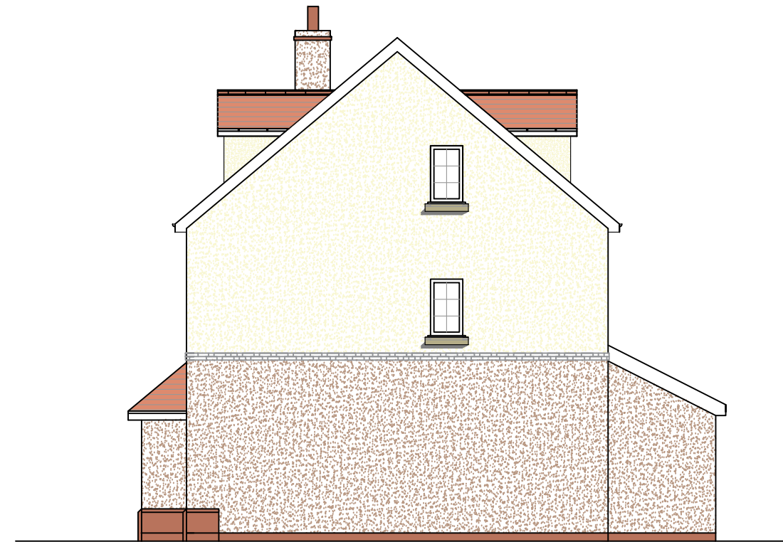
4 The Cherrington V1 Side Elevation D 1:100
