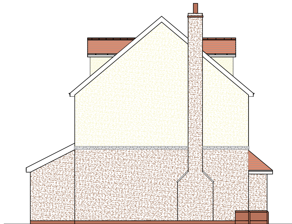
3 The Cherrington V1 Side Elevation C 1:100
