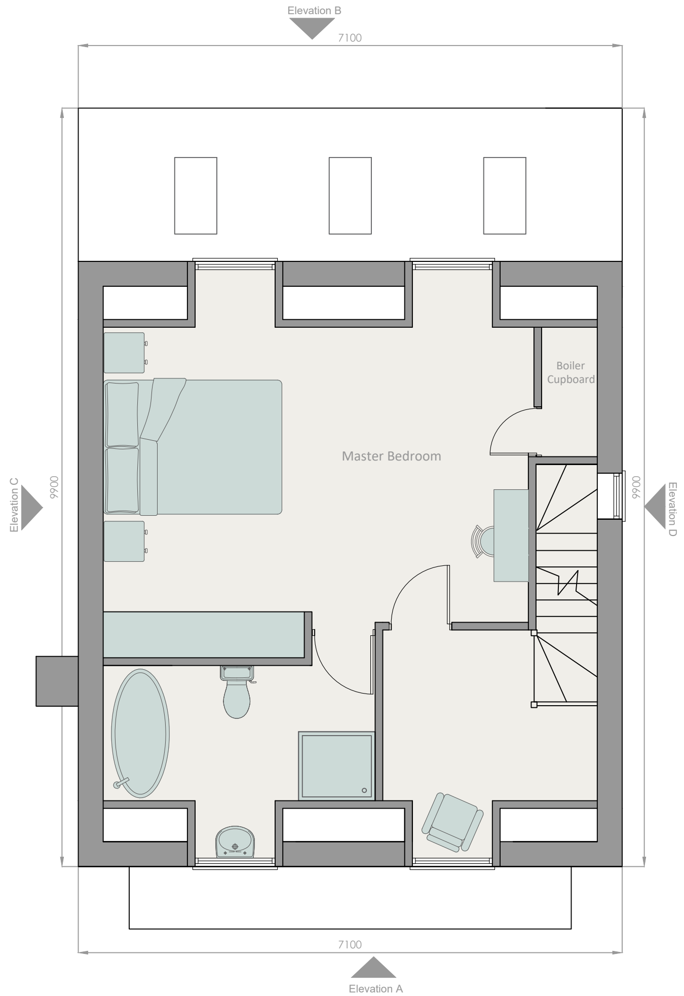
1 The Cherrington V1 Attic Floor Plan 1:50
