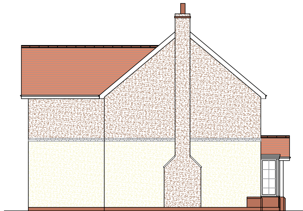
3 The Westbury V1 Side Elevation C 1:100
