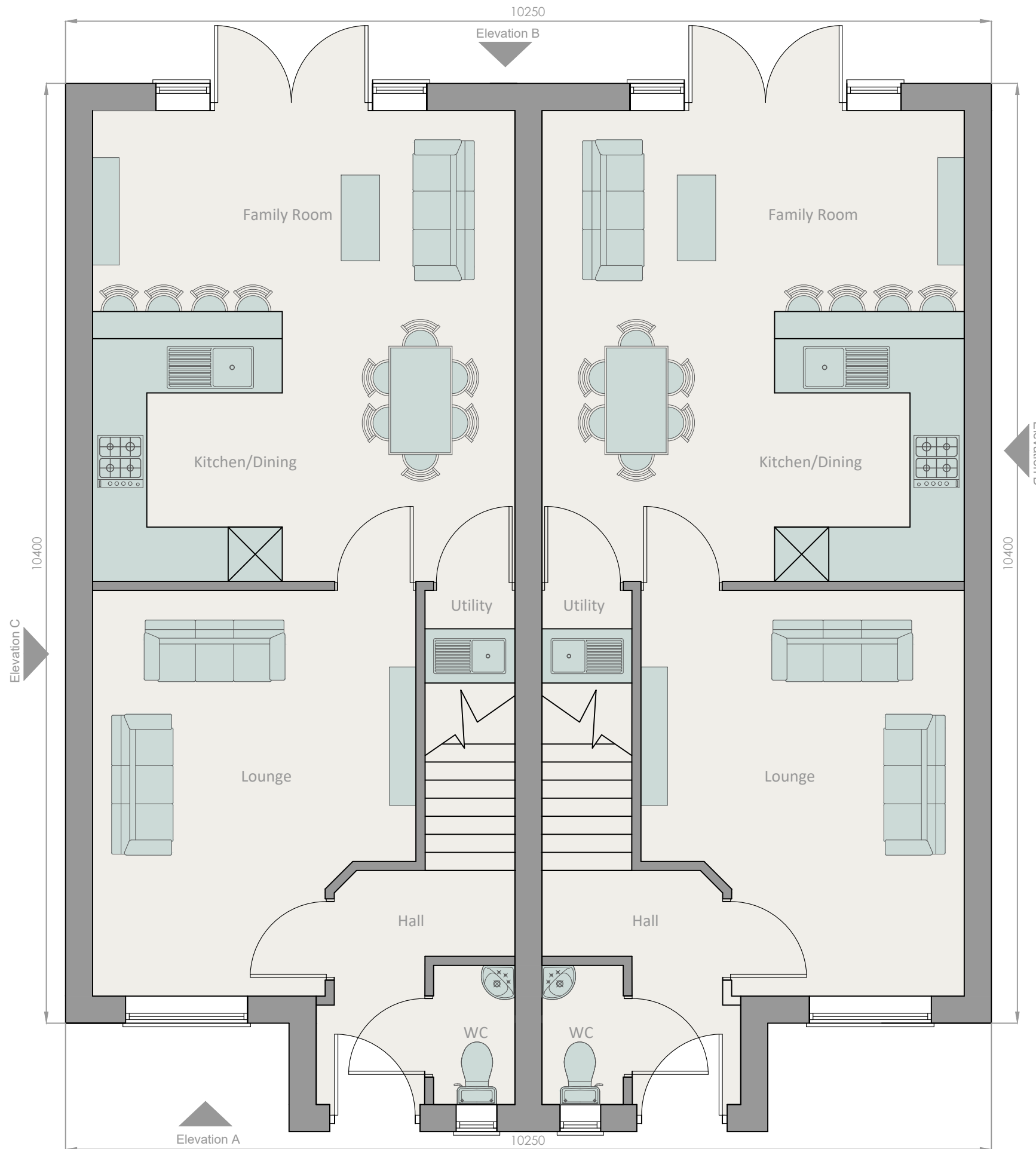
1 The AF1 and AF2 Ground Floor Plan 1:50
