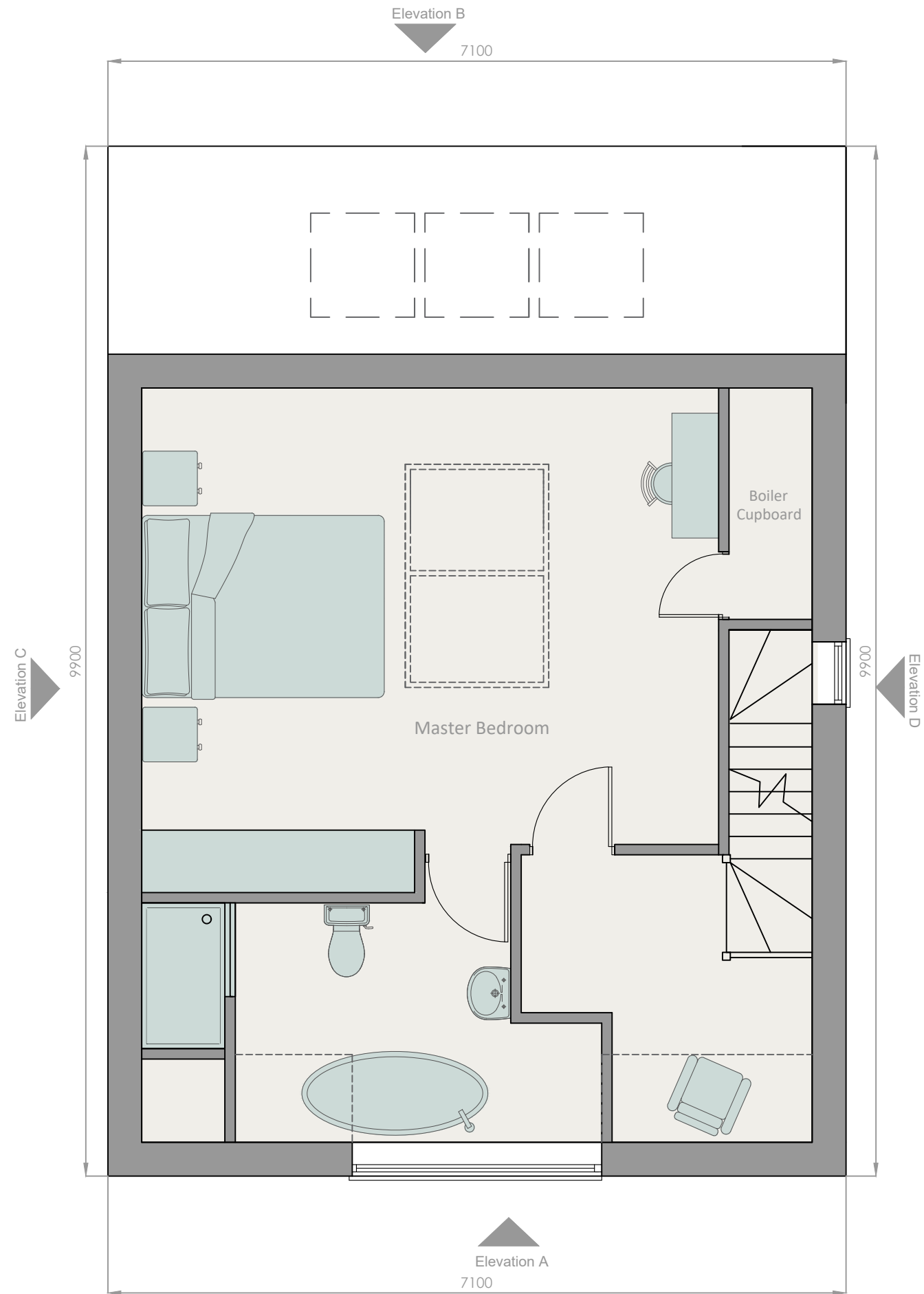
1 The Hathaway Attic Plan 1:50
