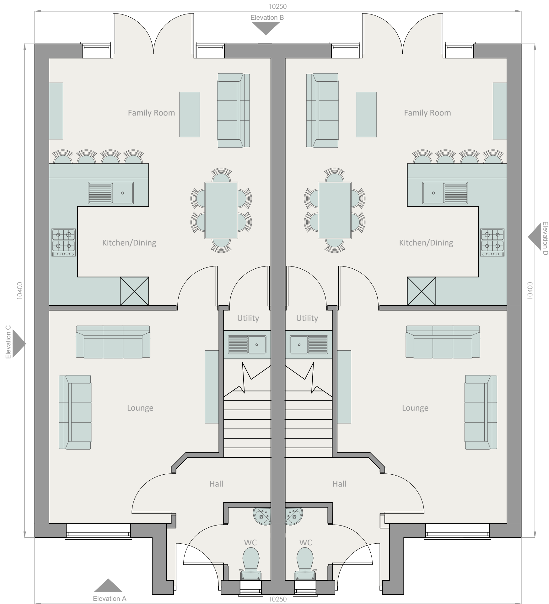
1 The AF1 and AF2 Ground Floor Plan 1:50
