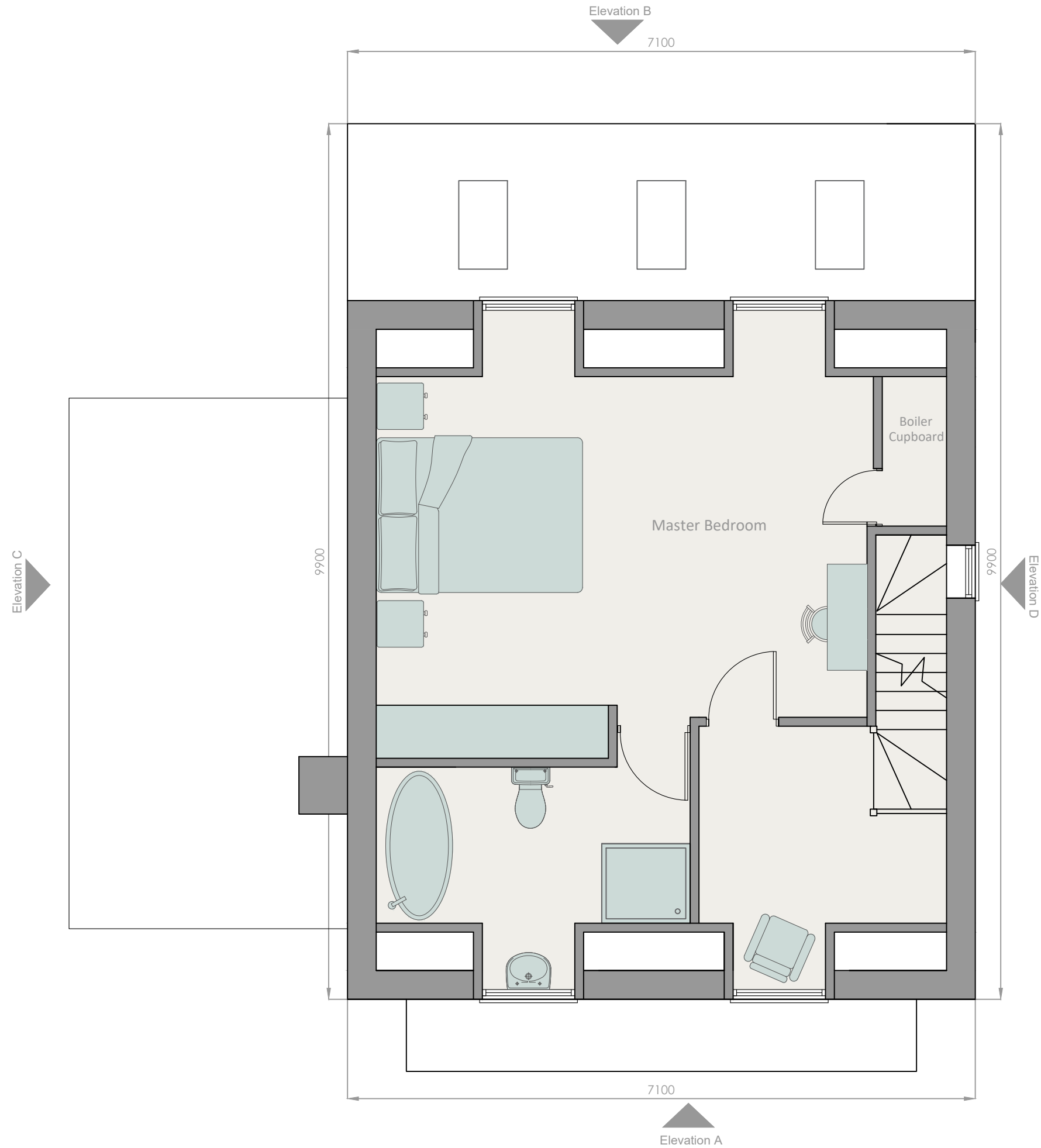
1 The Hathaway Attic Plan 1:50
