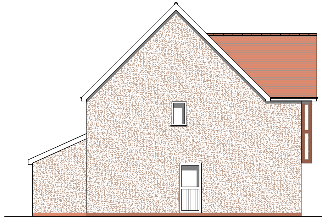
4 The Tudor Side Elevation D 1:100
