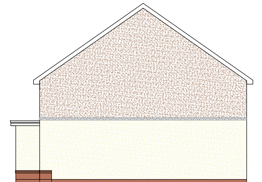
3 The AF1 & AF2 Side Elevation C 1:100
